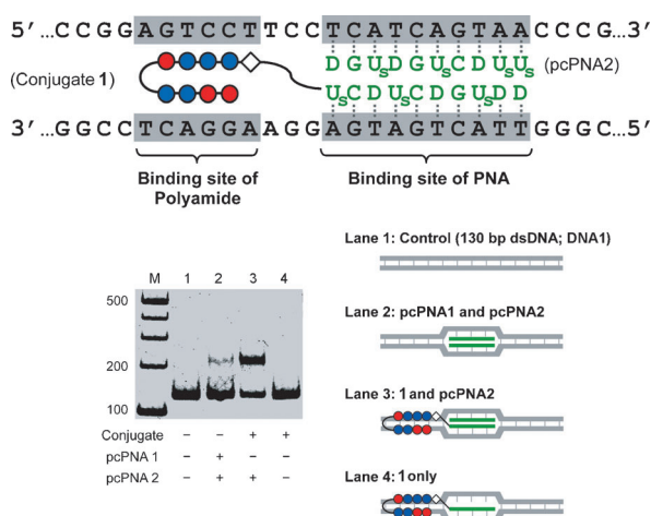
Figure 2. Gel-shift assay for binding of the combination of 1 and pcPNA2 to dsDNA. The pcPNA binding site (5'-TCATCAGTAA-3') and the polyamide binding site (5'-AGTCCTTCC-3') in the DNA1 are shown. Lane 1: DNA1 only; lane 2: DNA1 with pcPNA1/pcPNA2; lane 3: DNA1 with 1 /pcPNA2; lane 4: 1 only; M: 100 bp ladder. Invasion conditions: [DNA1] = 10 nM, [ 1 ] = 100 nM, [pcPNA1 or 2] = 100 nM, [HEPES] = 5 mM, and [NaCl] = 20 mM at pH 7.0 and 50 °C for 24 h.
